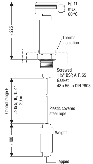
Level probe type NRG 21-51
