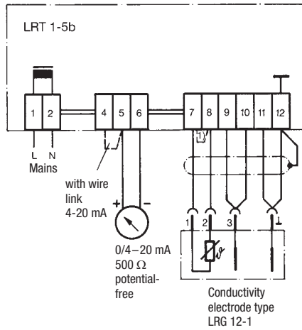
Conductivity transmitter type LRT 1-5b
