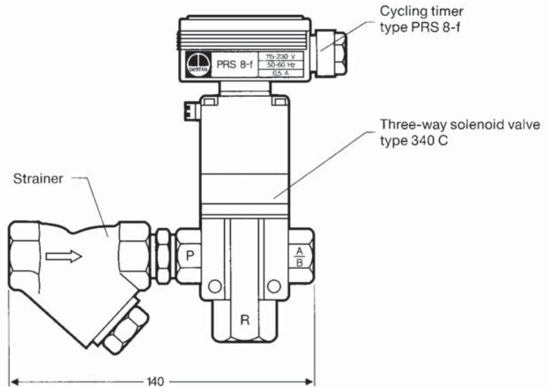
Dimensions of programme-controlled intermittent blowdown system
