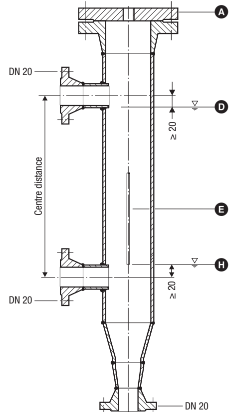
Fig. 3 External measuring pot
