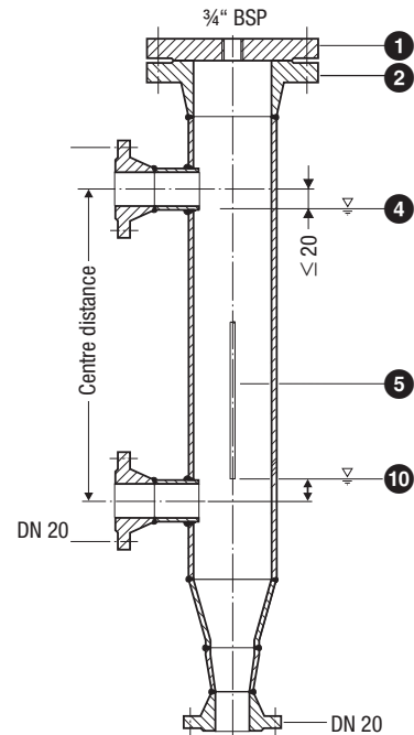
Fig. 4 External measuring pot
