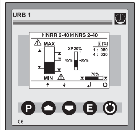
Example: Visual display of level monitoring system NRR 2-40
