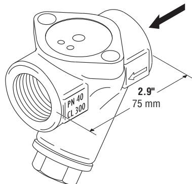
Flowserve Gestra Universal Connector
