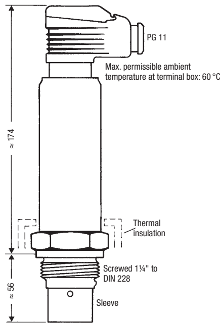
Conductivity electrode type LRG 12-1
