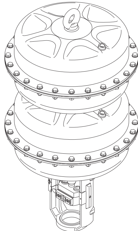
Actuator PB 3002 3000 m 2 Supply air: max. 6 barg Actuating force up to 60 kN
