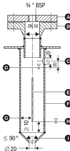
Fig. 2 Protection tube for installation of electrode inside the boiler
