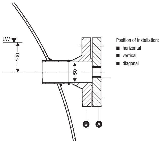
Fig. 2 Boiler standpipe, horizontal installation
