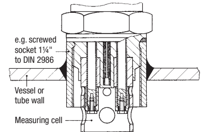
Installation of conductivity electrode in a screwed socket
