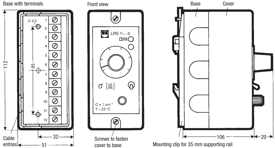
Dimensions of conductivity limit switch types LRS 1-5b, LRS 1-6b
