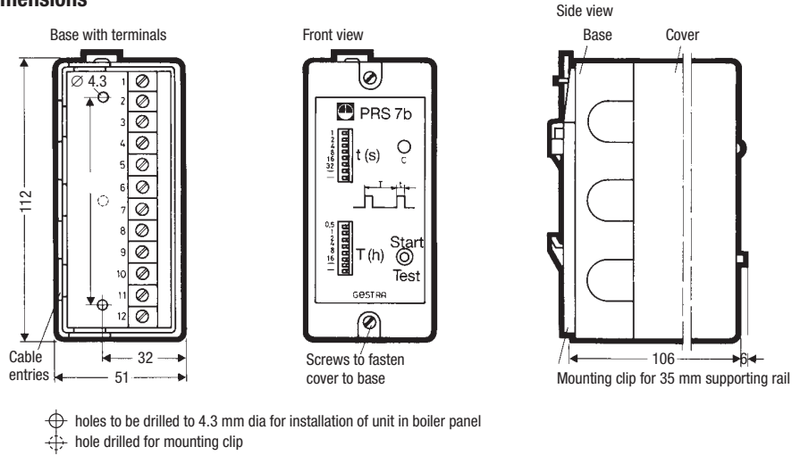
Cycling timer type PRS-7b as plug-in unit in plastic case, component part of programme-controlled blowdown system type TA 5
