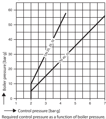
Control pressure (M)PA 46 / (M)PA 47
