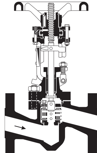
ZK 29/14, DN 25 mm (1") with flanged ends
