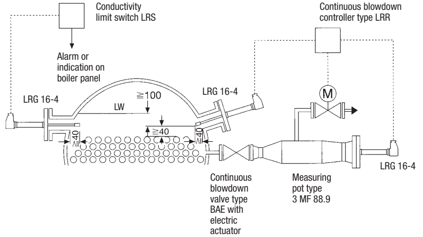
Left-hand side horizontal installation of conductivity electrode type LRG 16-4 in a boiler drum, right-hand side installation of LRG 16-4 inside the boiler and outside in a measuring pot
