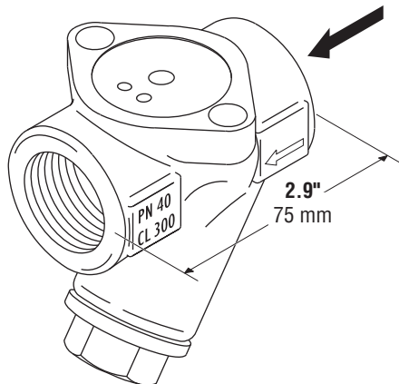
Flowserve Gestra Universal Connector
