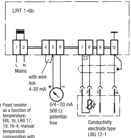
Conductivity transmitter type LRT 1-6b
