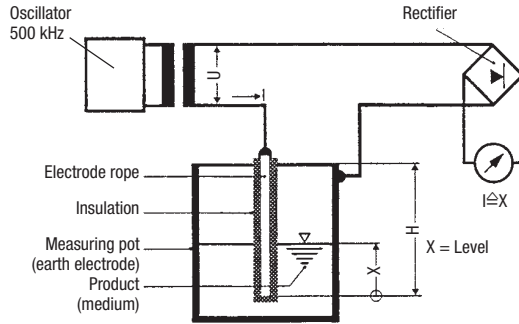
Schematic diagram of level probes type NRG 21-...
