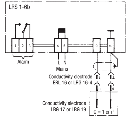
Wiring diagram for conductivity limit switch type LRS 1-6b, illustrated position of contact: relay de-energized, i.e. alarm
