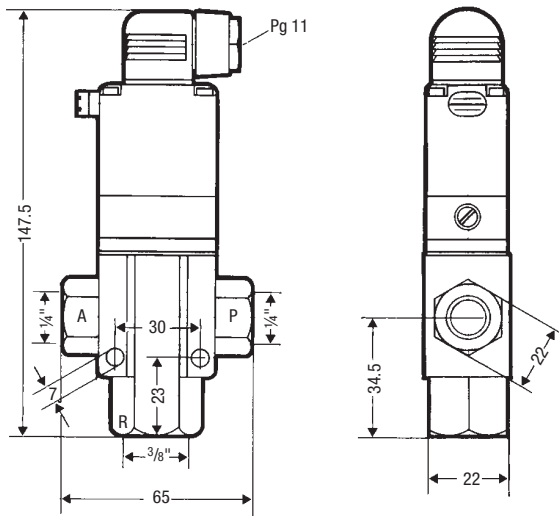
Three-way solenoid valve type 340 C, 1/4", component part of programme-controlled blowdown systems types TA 5, TA 4
