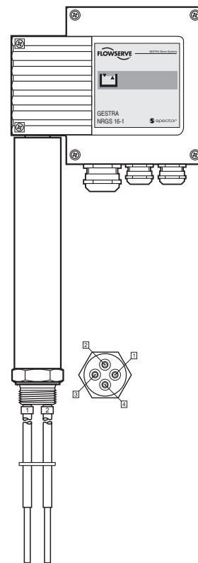
Wiring Diagram Fill control
