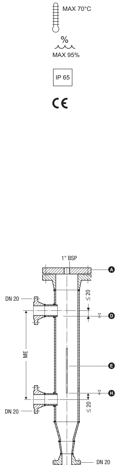
Fig. 3 External measuring pot
